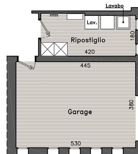
Piano terra
